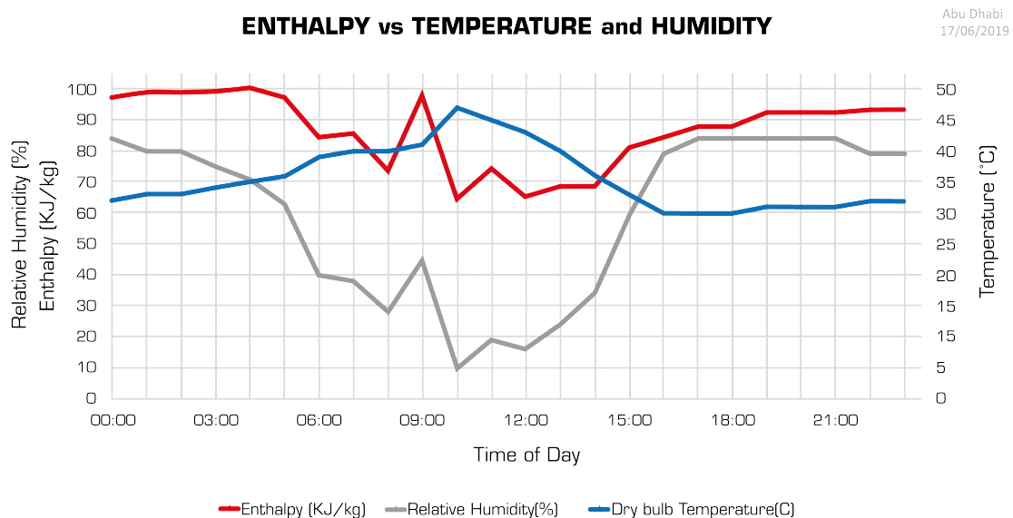
Image 2: The chart shows the measurements of temperature and humidity done in Abu Dhabi on the 17th of June in 2019. Accompanied is the corresponding enthalpy.
